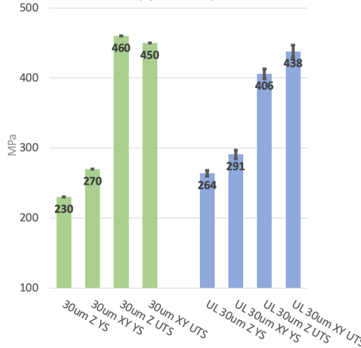
OEM 30um (spec sheet) vs. UL HPS 30um
